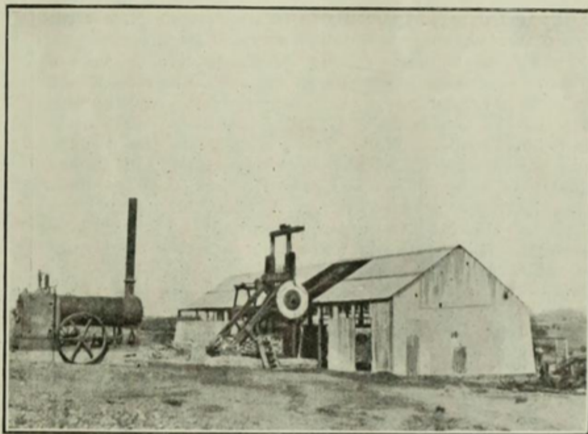
EDENDALE FIVE-STAMP MILL.
